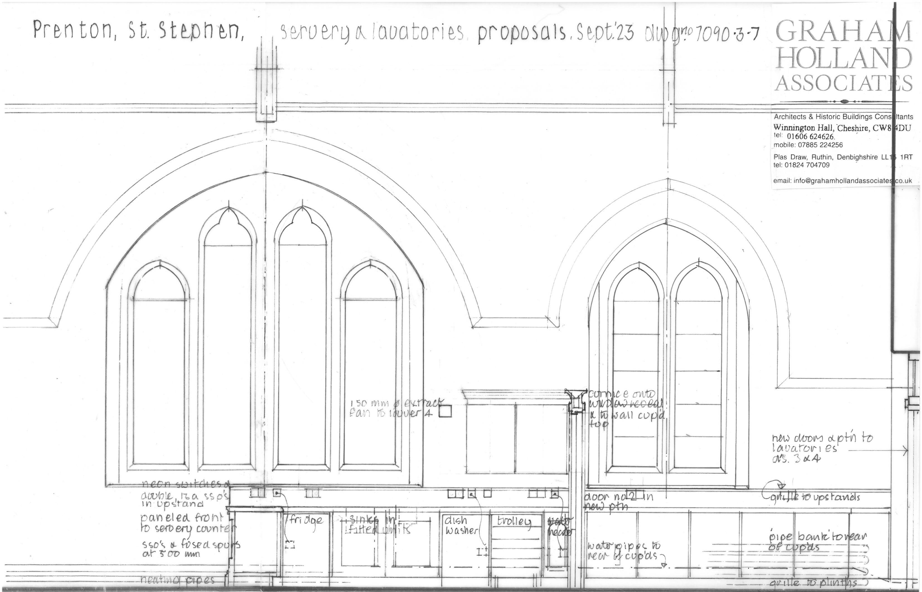
elevation section in the south aisle, looking south 1:25 @ A3 check all details & dimensions on site
